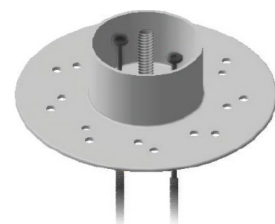
[P/N 2001] Universal Base and Duro-Last Approved Fastener
