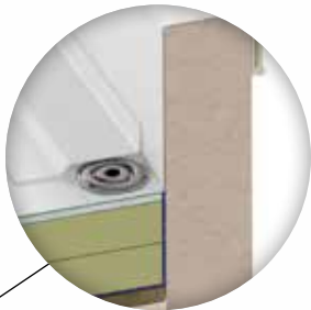
Custom-Fabricated Wall Flashing
