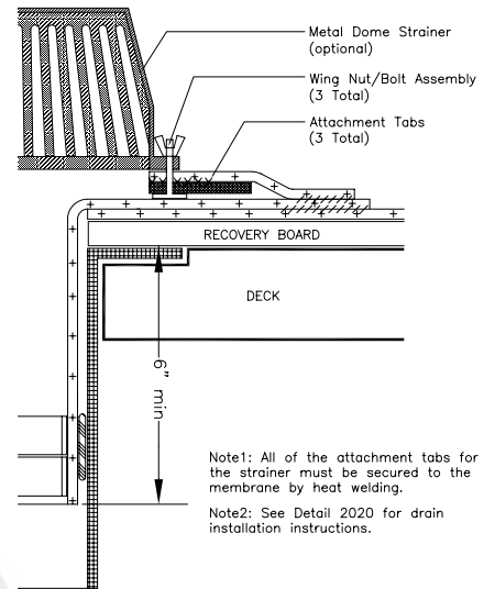
2021 NTS DRAIN BOOT W/DL DOME STRAINER New Construction or Reroof © COPYRIGHT 2003
